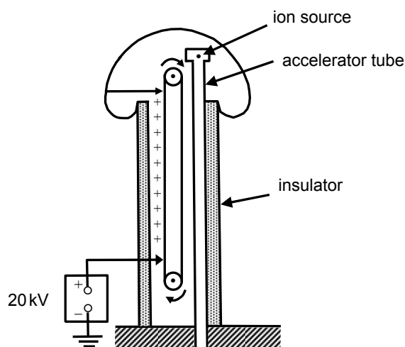
Figure 10 Vertical cross-section of a Van de Graaff generator
