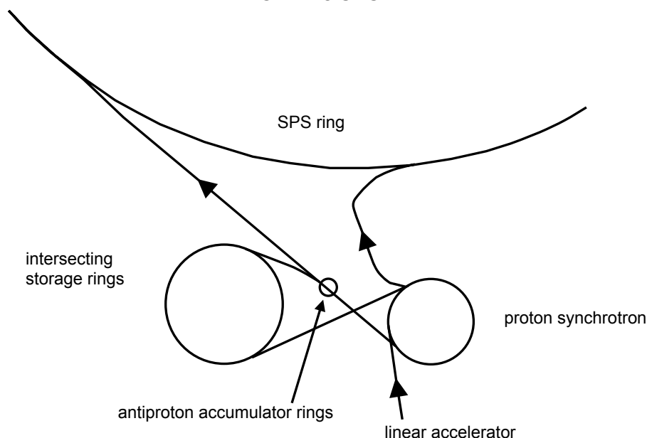
Figure 15 CERN's SPS
