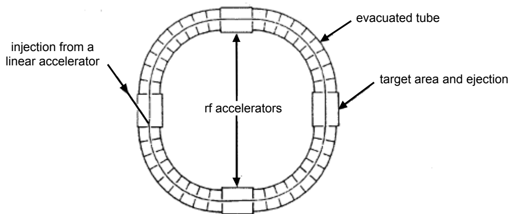
Figure 12 The Synchrotron
