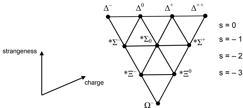
Figure 17 Predicting the \Omega^- particle
